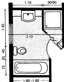
⑨ Bathroom with separate shower
